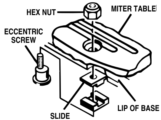
Figure 54: Miter Fence Alignment
