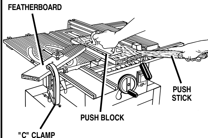
Figure 43: Making A Non-Through Cut
