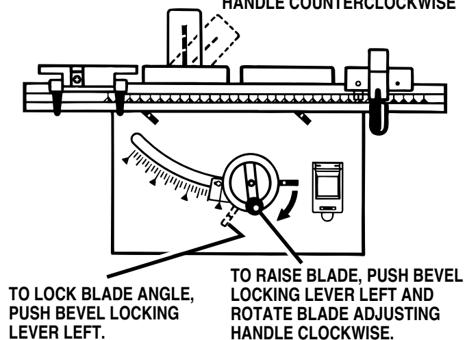
Figure 25: Blade Movement Directions
