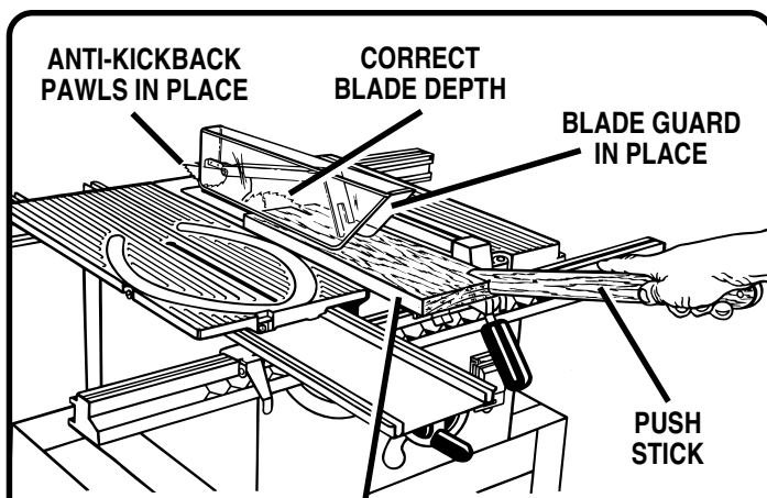
Figure 29: Anti-kickback Practices
