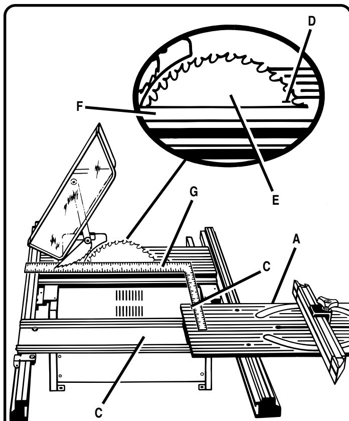
Figure 50: Miter Table Alignment
