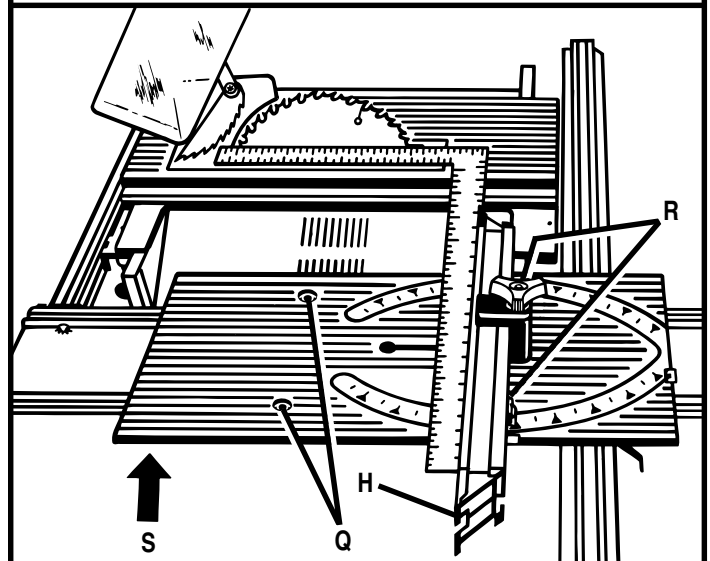
Figure 55: Miter Fence Alignment
