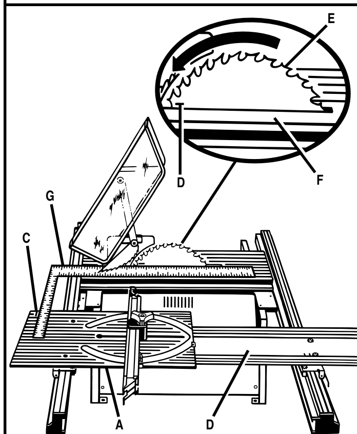
Figure 51: Miter Table Alignment
