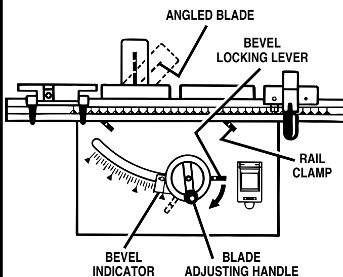
Figure 33: Angling the Blade
