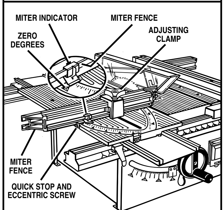
Figure 56: Quick Stop
