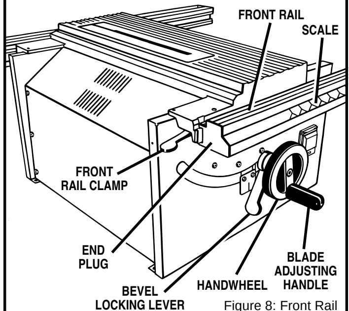
Figure 8: Front Rail
