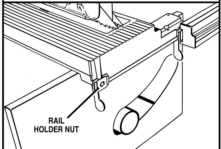
Figure 8: Front Rail
